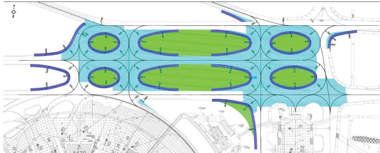
REDESIGN OF TAXIWAY DELTA – Final configuration End of January 2021
